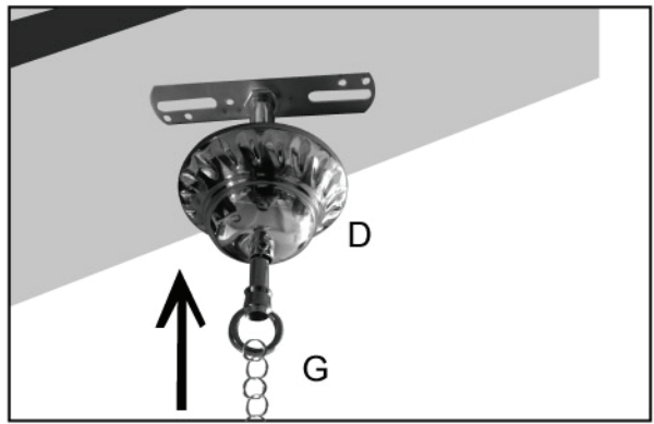
Step 4: Insert the Mounting Cap Bolt through Mounting Cap.
