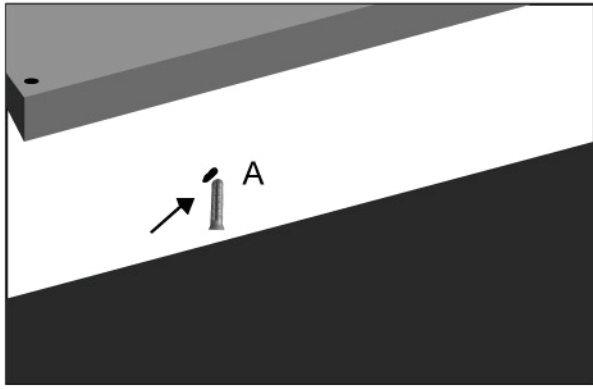
Step 1: Determine position light will hang and mark locations on ceiling so mounting chains hang straight. Try to hit a ceiling joist. If not, use Bracket as template, mark and drill holes for Plastic Anchors.
