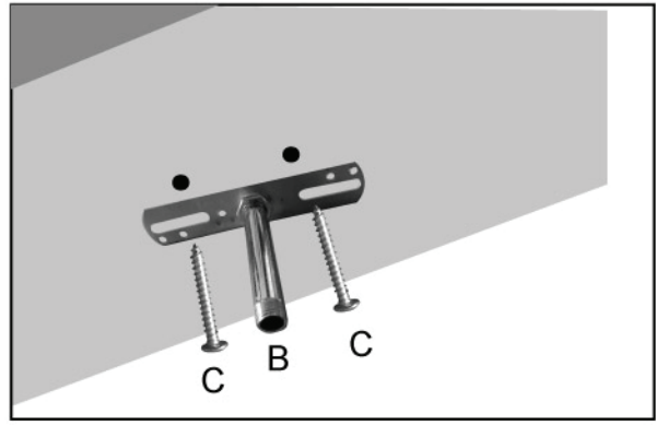
Step 2: One Bracket will screw to the ceiling. *Note: at least one Bracket will mount to an existing or installed electrical box to provide power. Please consider this when selecting location.
